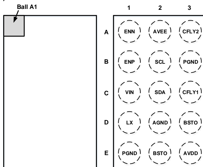
Figure 1, Pin Assignments of TCS3514
