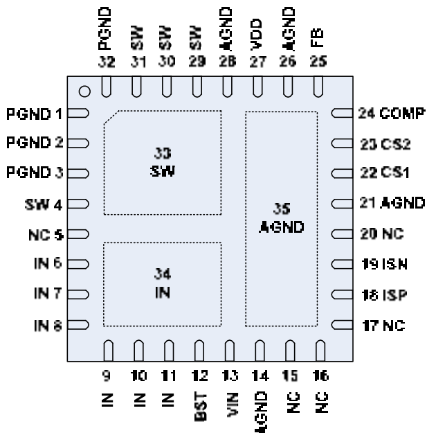
Figure1 Pin Configuration of TCS4462(TopView)
