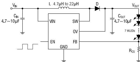
Figure 1. Basic Application Circuit
